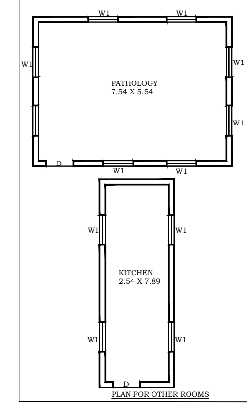
BUILT-UP AREA CALCULATION
