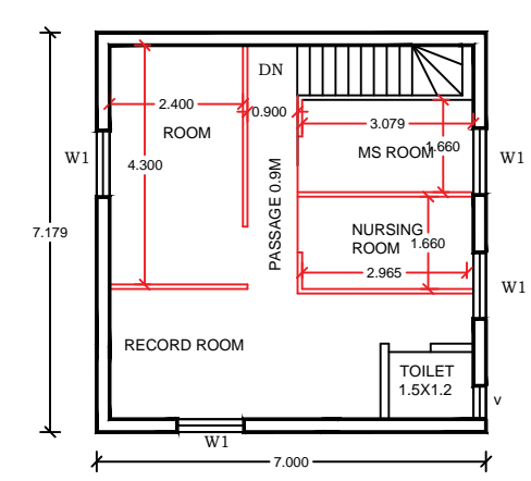
1ST FLOOR PLAN SCALE :1:100
